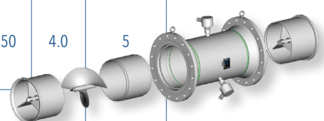
3 Piece Design ≥ 14 "
